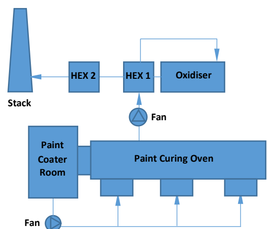
Figure 1.0: Typical CCCL Thermal System
